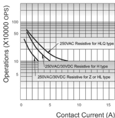
EDURANCE CURVE
